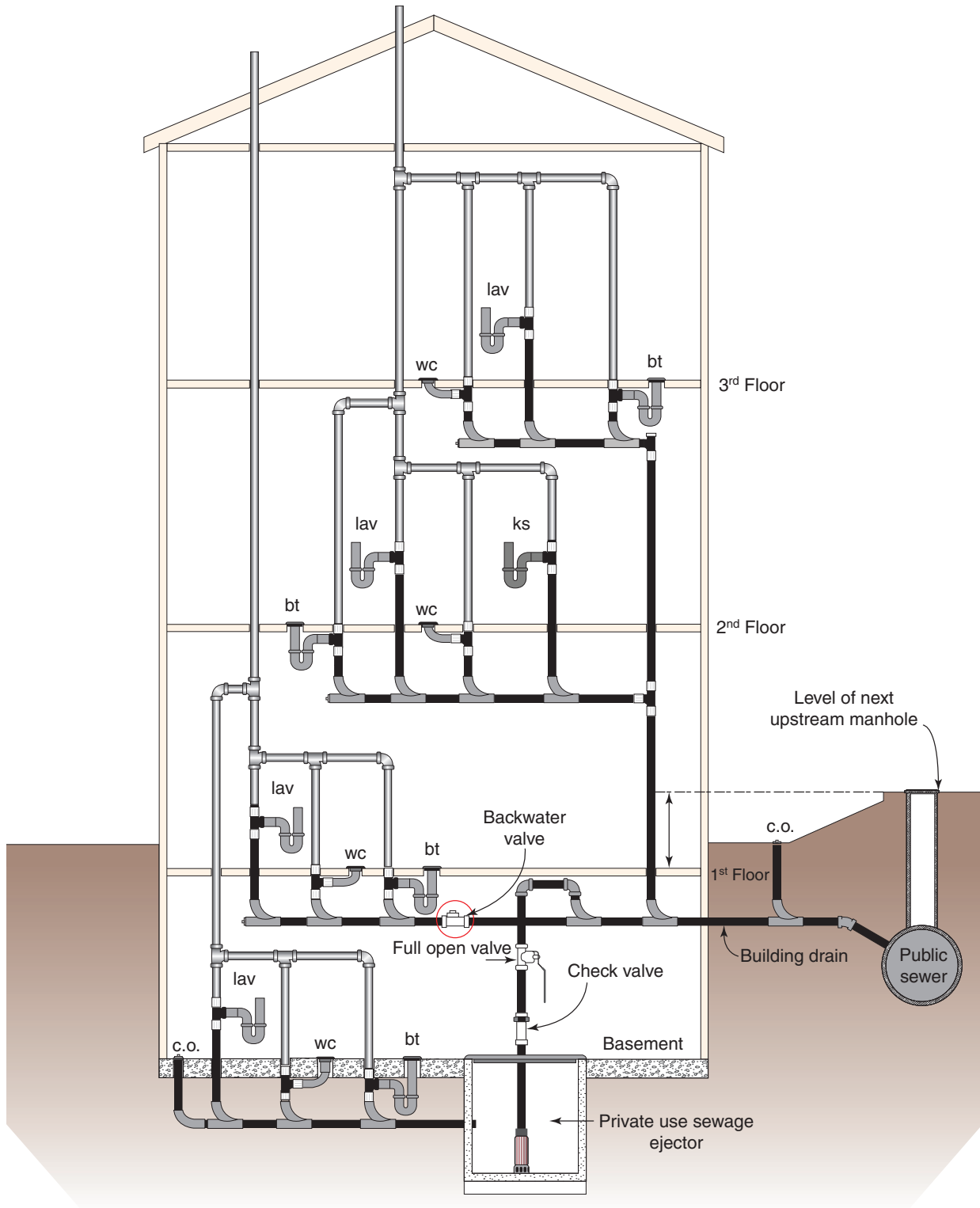
Figure 10: Sewage Backflow
