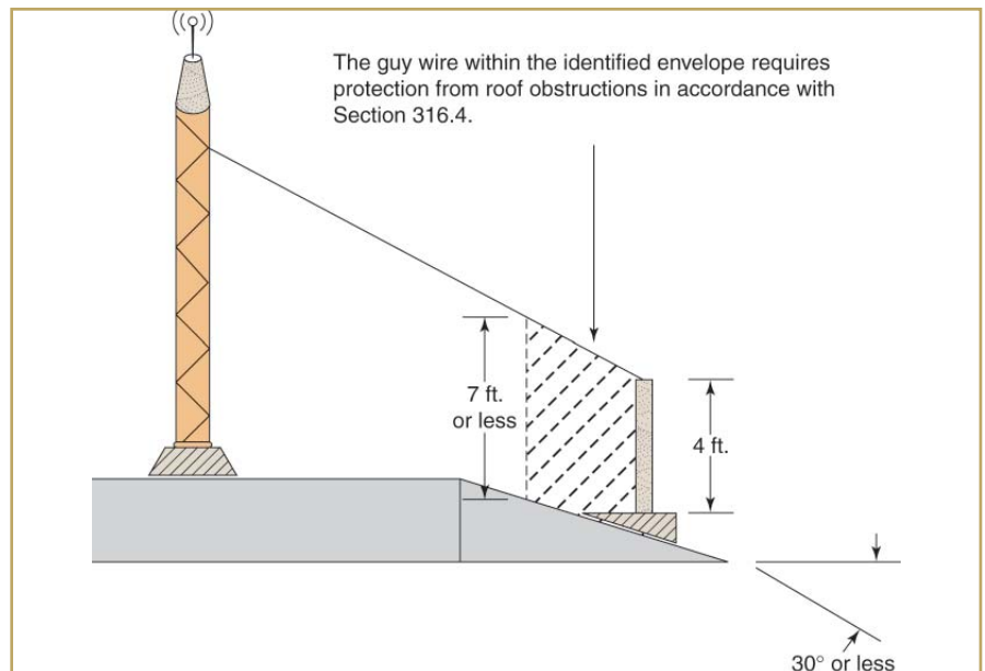
FIGURE 3-9 Obstructions on rooftops must be protected so as not to create a hazard to fire-fighting operations.
